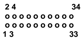
DIAGRAM 2 Pin connections of the disk drive connector (Front View).
